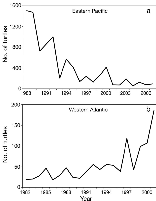
Fig. 1. Dermochelys coriacea . Population trends at representative nesting beaches in; (a) the eastern Pacific (Parque Nacional Marino Las Baulas, Costa Rica; P. Santidrián Tomillo, G. Blanco, J. R. Spotila, & F. V. Paladino unpubl. data) and (b) the western Atlantic (Sandy Point National Wildlife Refuge, St. Croix, US Virgin Islands; Dutton et al. 2005)
